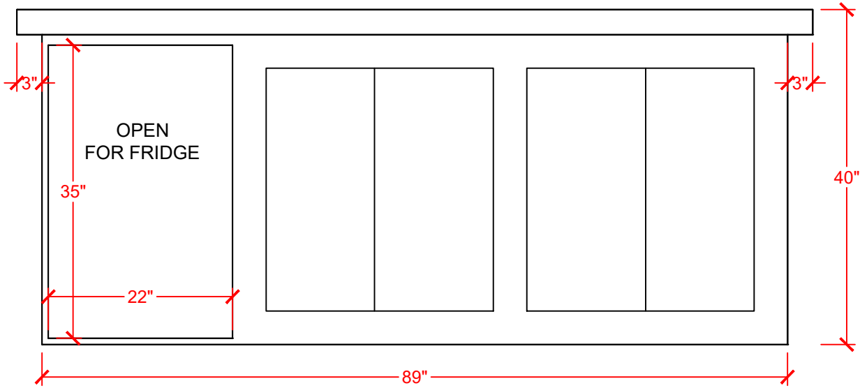
FRONT ELEVATION
