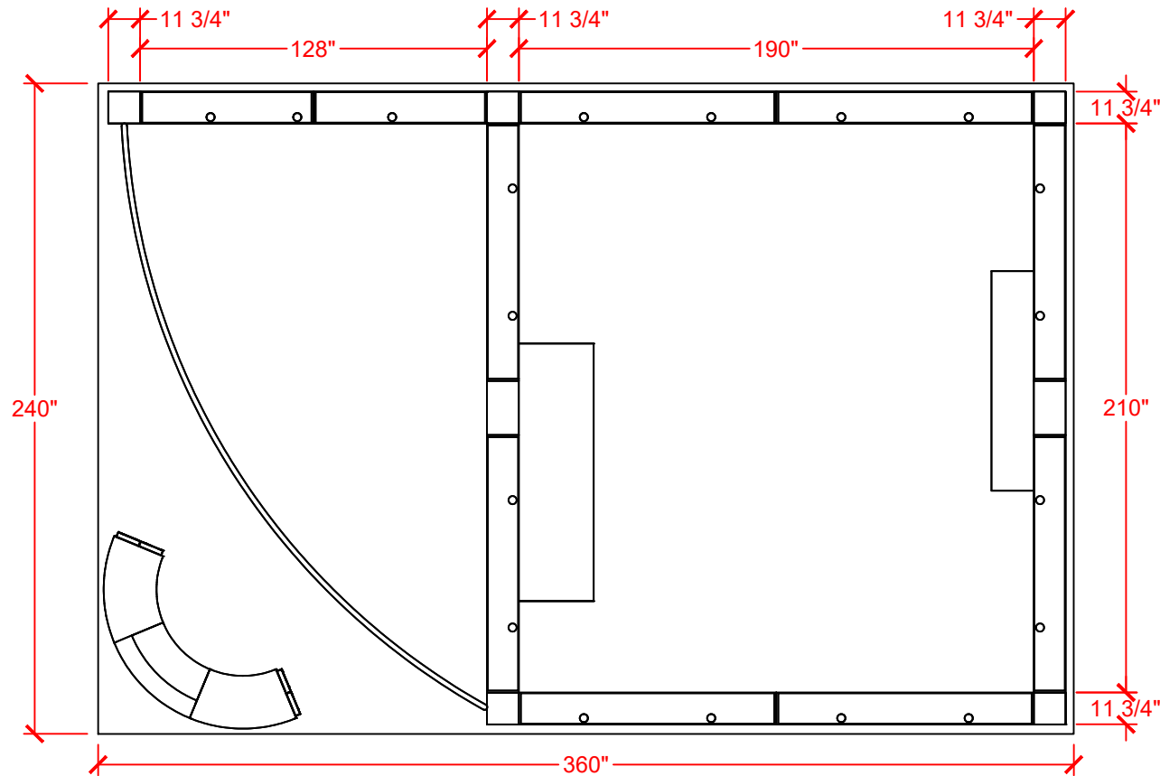
PLAN VIEW SCALE: 3/16" = 1'
