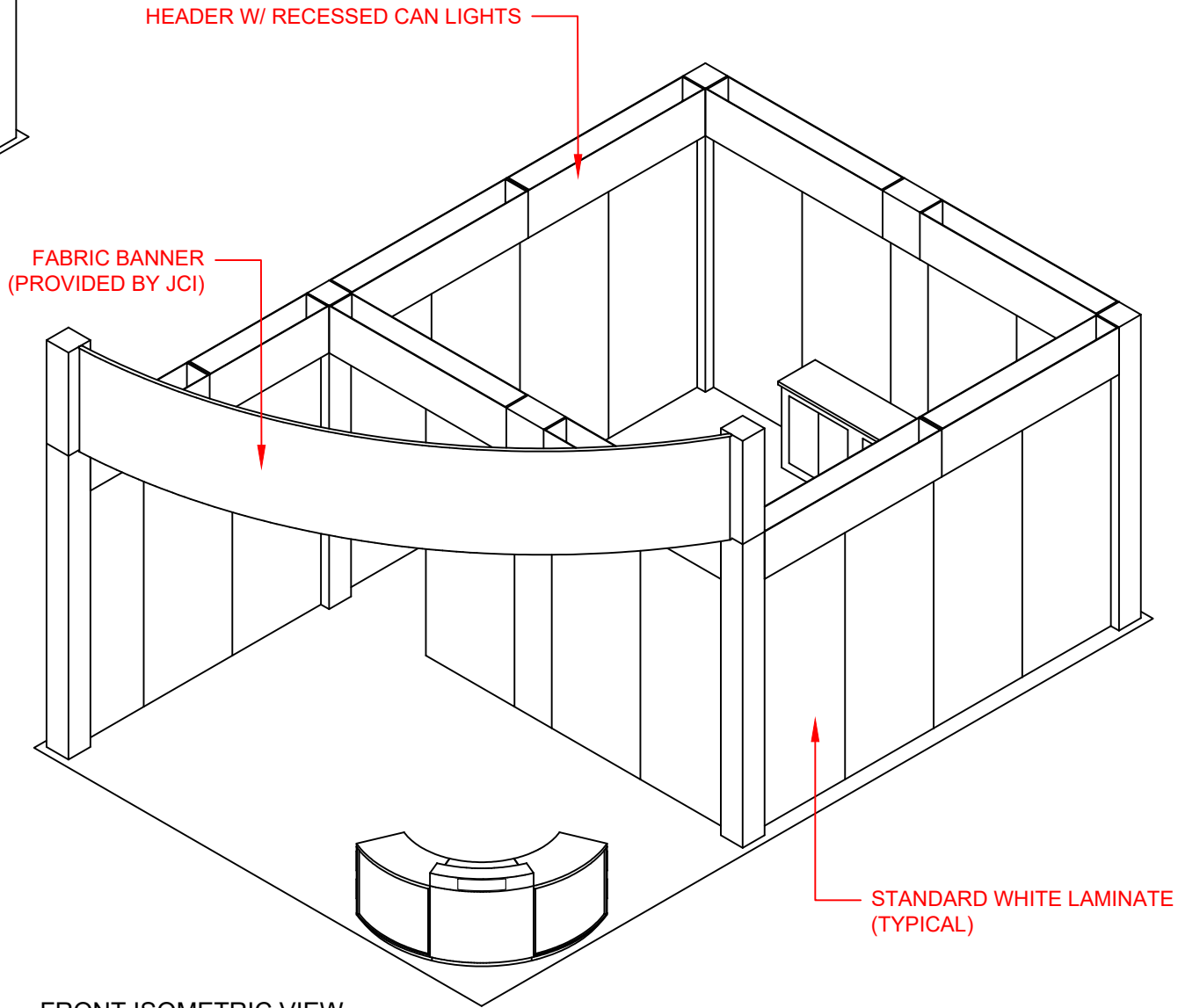
FRONT ISOMETRIC VIEW
