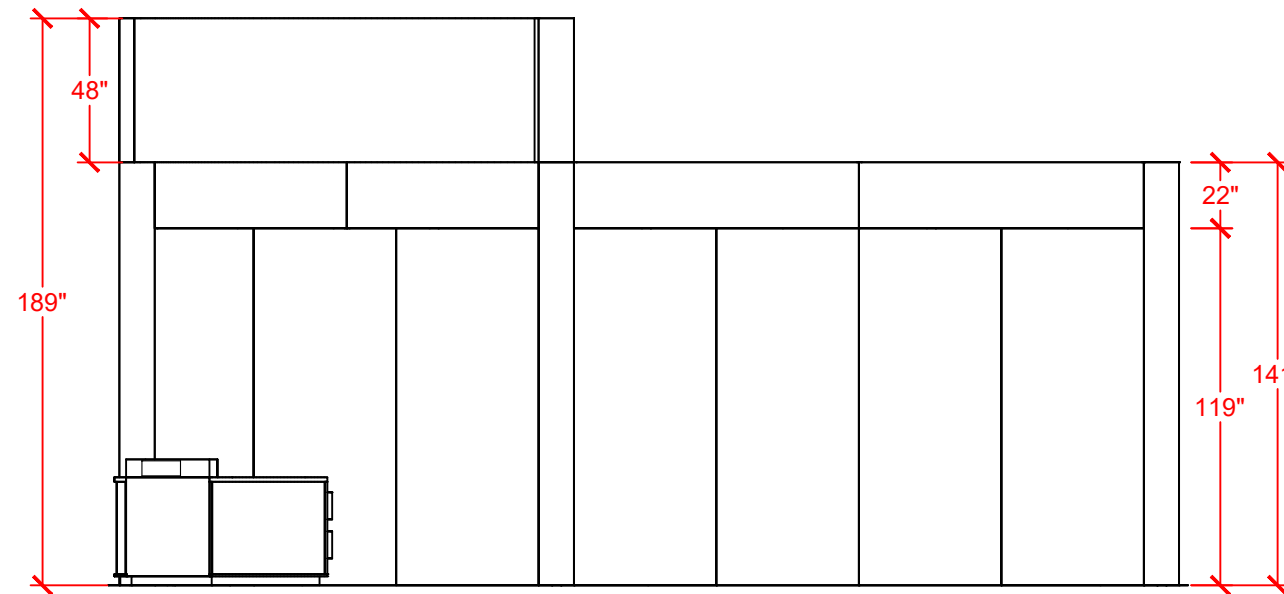
FRONT ELEVATION SCALE: 3/16" = 1'
